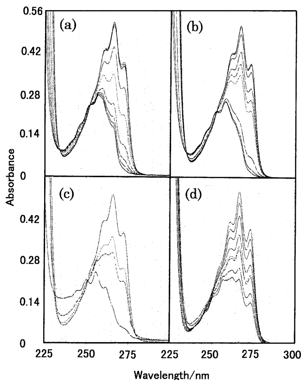
Fig. 1. UV spectral changes by the acid-base reaction of PB (a, b) and by the reaction of PB with F - (c, d) in water (a, c) and in 60% MeOH (b, d). C_{\text{PB}} = 10^{-3} mol dm -3 . -\log [\text{H}^+] = 6-11 (a, b), 3.0 (c, d). C_{\text{F}}/\text{mol dm}^{-3} = 0 (a, b), 0-10^{-2} (c, d).
